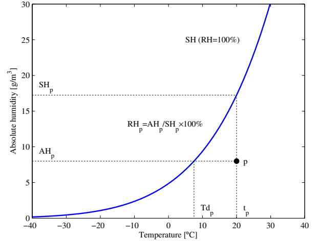
Fig. 1. Relationship between the following weather variables: temperature ( t ), relative humidity ( RH ), absolute humidity ( AH ), saturated humidity ( SH ), and dew point ( T_d ) (at constant barometric pressure).
